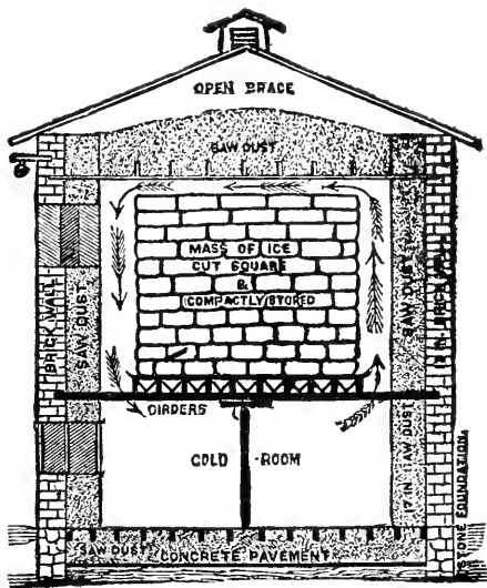
Refrigerating House.
